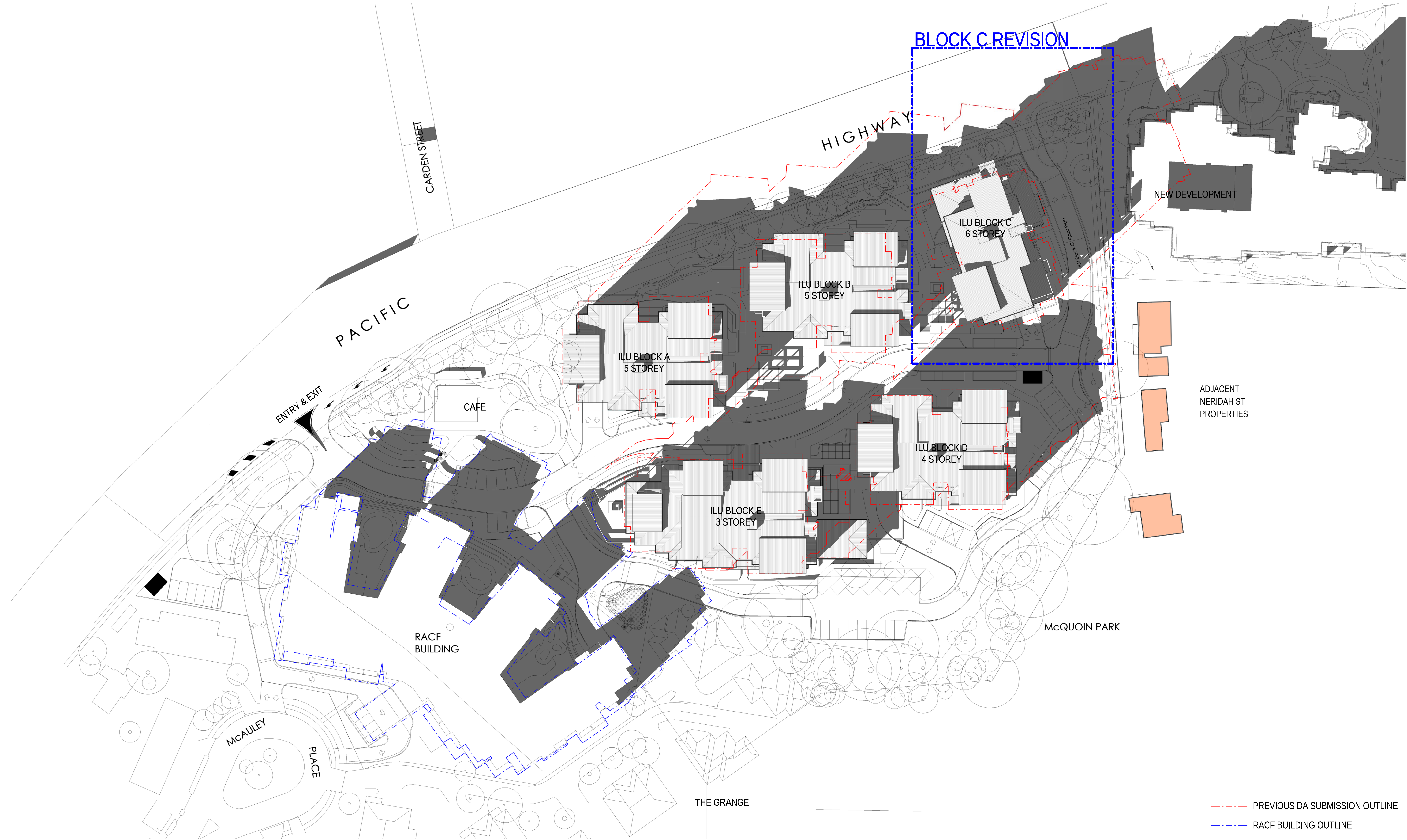
1 21 JUNE 3PM - SHADOW DIAGRAM PLAN VIEW SCALE 1 : 400
